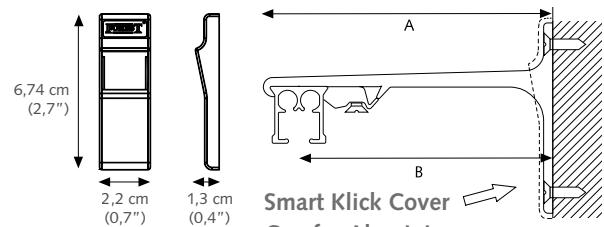
SK Wall bracket aluminium double
